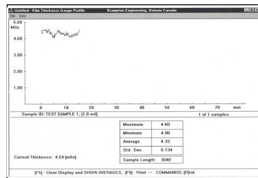
The Model DAQ-MIC Main Screen Showing Thickness Profile Data
